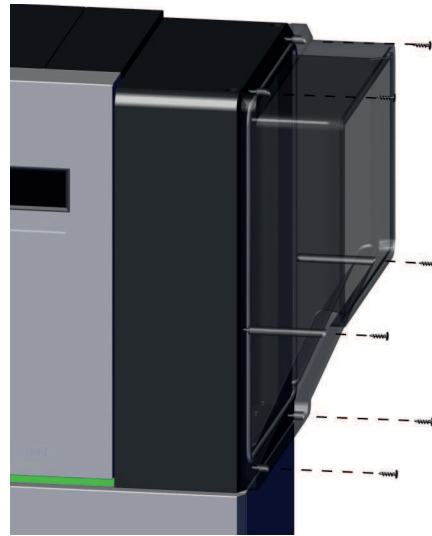
Abb. 11: Adapter befestigen
